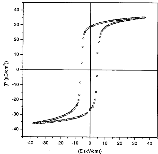
FIG. 3. Polarization ( P ) vs electric-field ( E ) curve for \langle 001 \rangle textured PMN-32PT.
